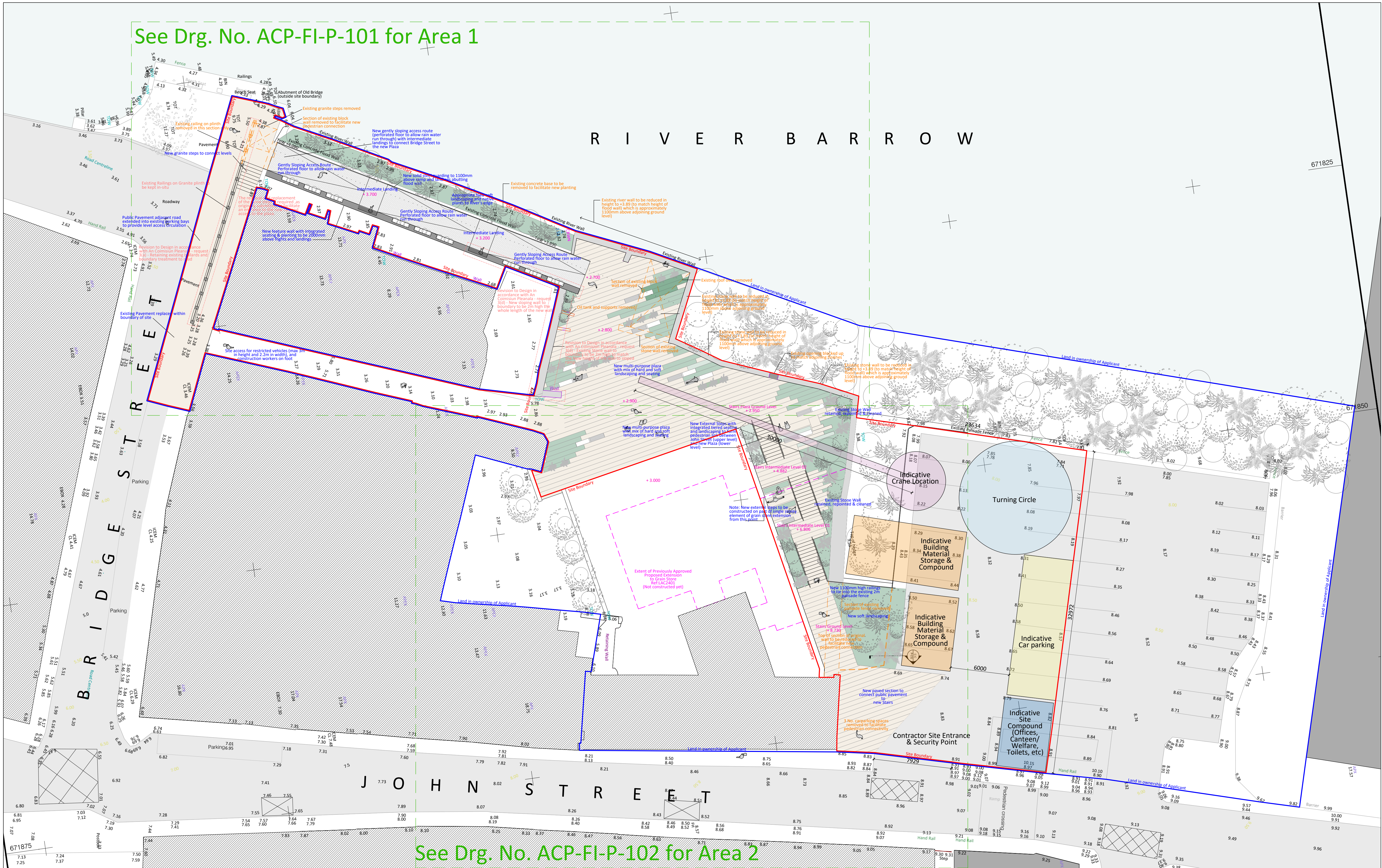
01 Site Layout Plan (Entire Site) As Proposed Scale: 1:200
